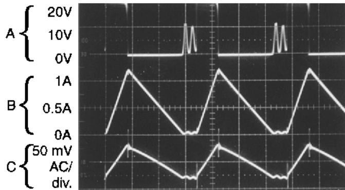
Figure 21. Horizontal Time Base: 2 \mu\text{s} /div.
