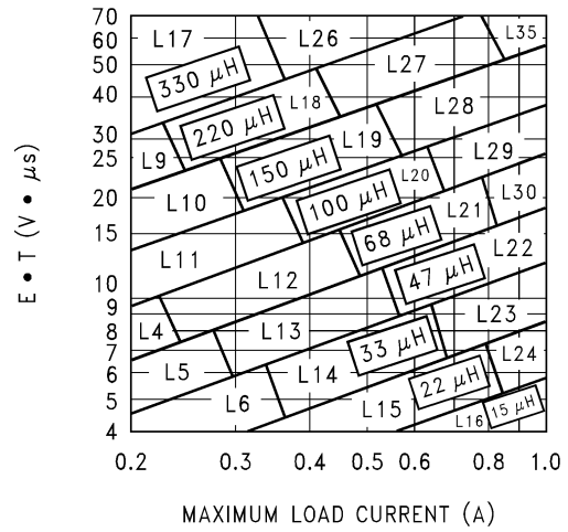
Figure 28. LM2598-ADJ
