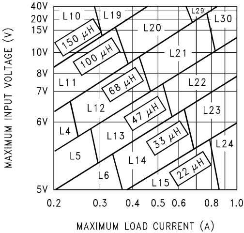
Figure 25. LM2598-3.3
